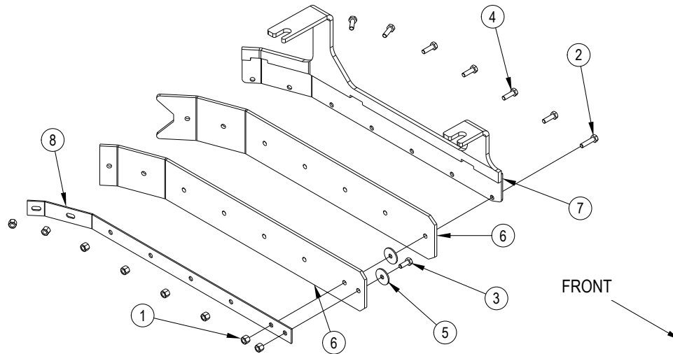
56601468 - Left Skirt Assy
