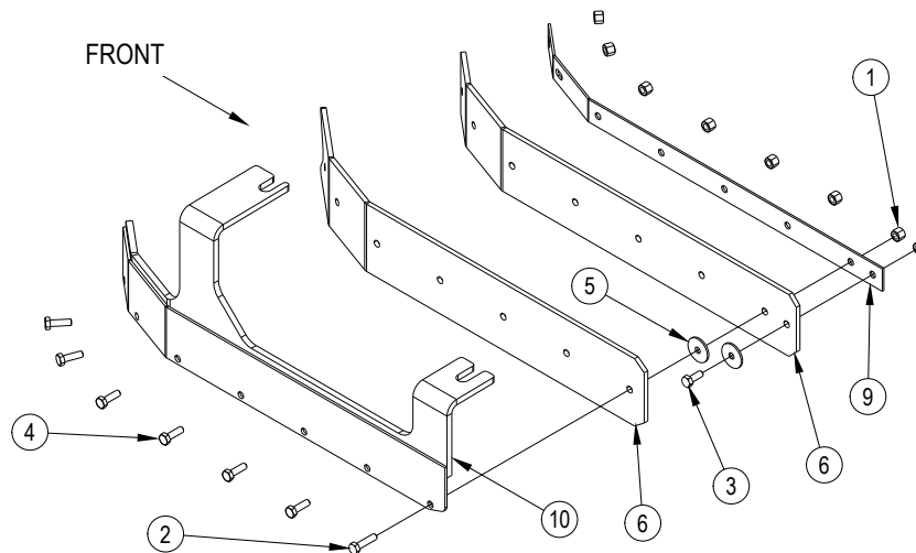
56601476 - Right Skirt Assy
